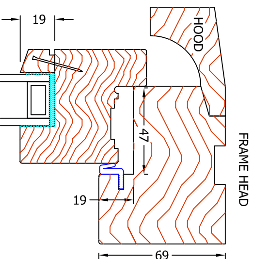
SECTIONS THROUGH STORMPROOF WINDOW CONSTRUCTION SCALE 1-2
