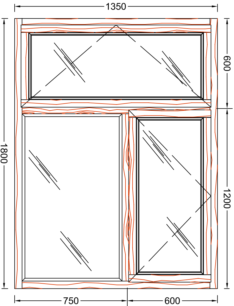
EXAMPLE OF WINDOW CONFIGURATION
